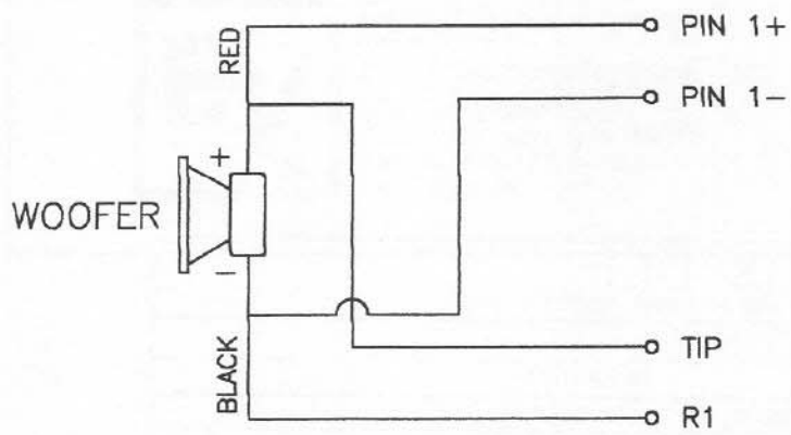
SCHEMATIC DIAGRAM
